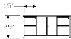
Storage Cabinet Full Back Panel
